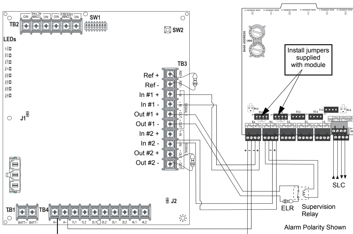
Figure 5.4 Wiring for Split Alarm Mode
