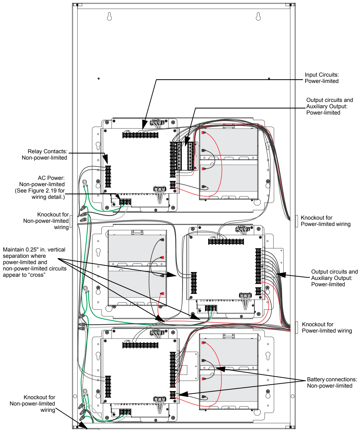
Figure 2.18 Power-Limited Wiring Example: EQBB-D4 with HPFF12CM(E)
