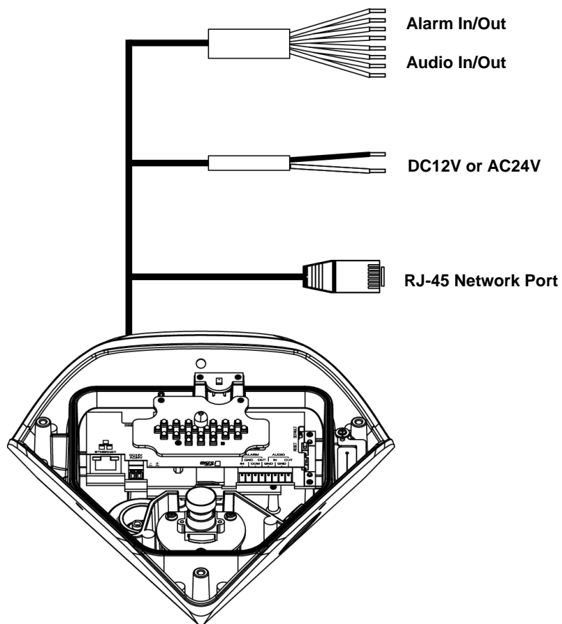
FIGURE 2 - 3: CONNECTING THE WIRES
