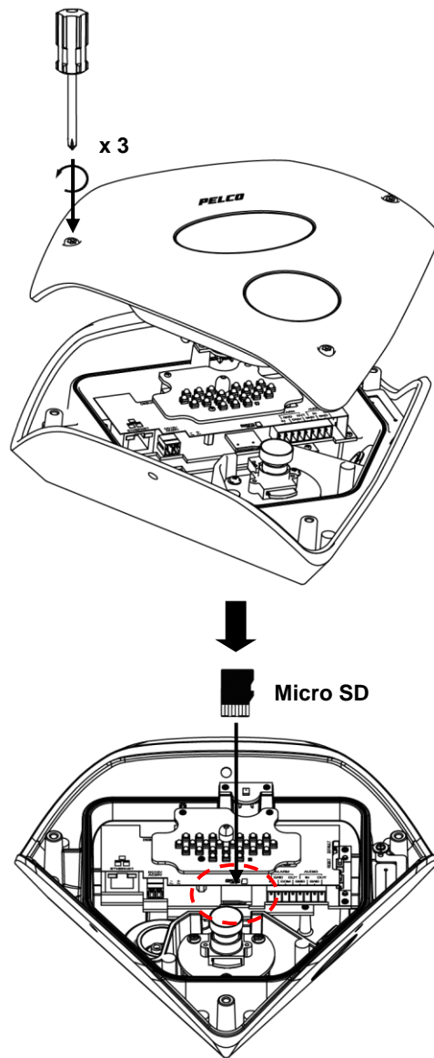
FIGURE 2 - 1: DISASSEMBLING THE CAMERA
