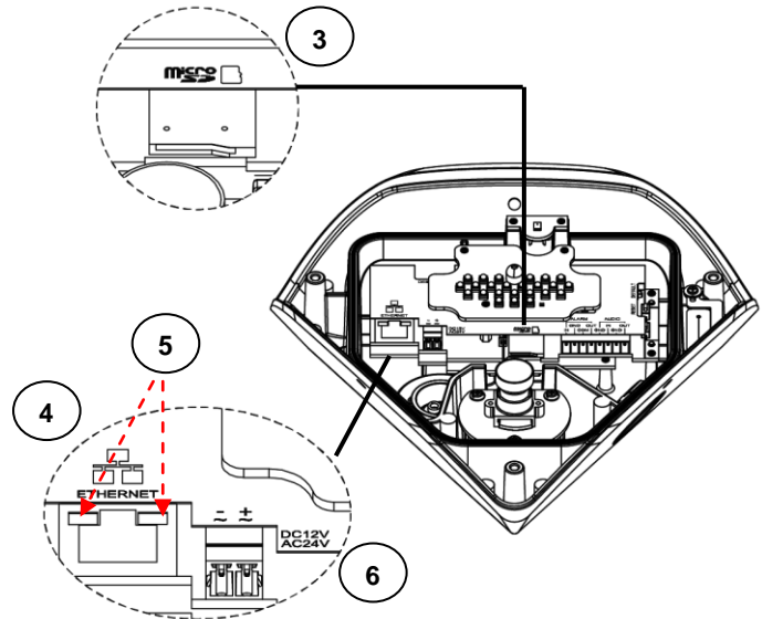
FIGURE 1-3: CAMERA CONNECTIONS AND FEATURES 2/4
