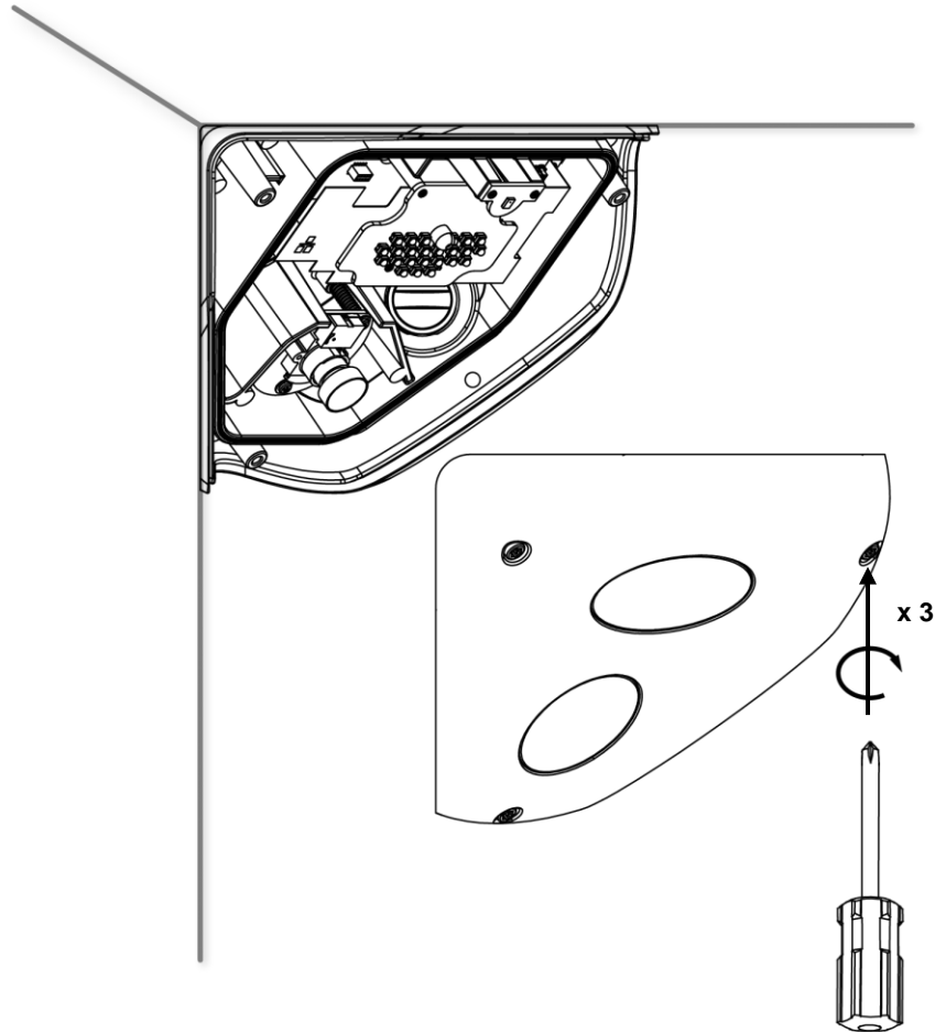
FIGURE 2 - 6: COMPLETING THE INSTALLATION
