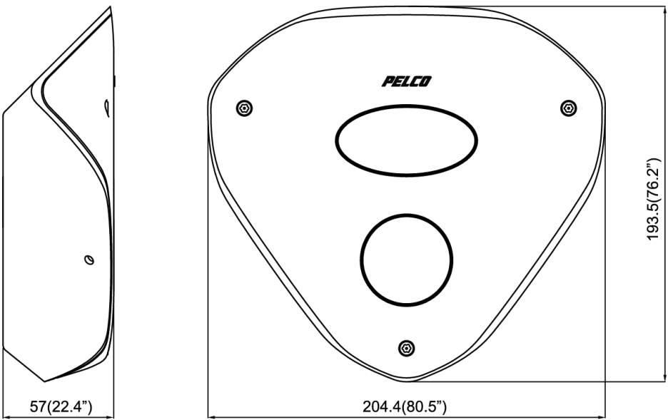
CORNER MOUNT HIGH SECURITY CAMERA
