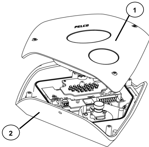
FIGURE 1-2: CAMERA CONNECTIONS AND FEATURES 1/4
