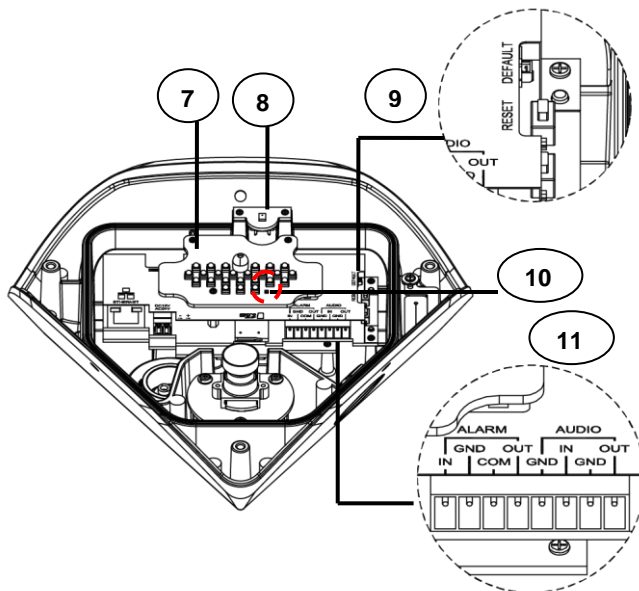
FIGURE 1-4: CAMERA CONNECTIONS AND FEATURES 3/4
