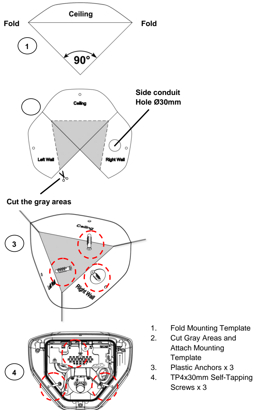
FIGURE 2-4: MOUNTING THE CAMERA
