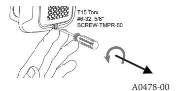
FIGURE 12. SURFACE MOUNT BACK BOX UP ARROW
