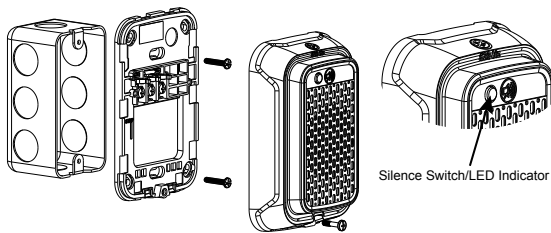
FIGURE 9. COMPACT WALL MOUNT LOW-FREQUENCY SOUNDER SOUNDER WITH LED ALARM INDICATOR AND SILENCE SWITCH, IN JUNCTION BOX
