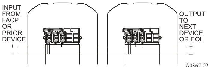
FIGURE 1. WIRING DIAGRAM
