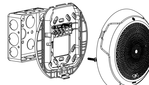
FIGURE 5. CEILING MOUNT LOW-FREQUENCY SOUNDER WITH JUNCTION BOX (SOUNDER-ONLY SHOWN)
