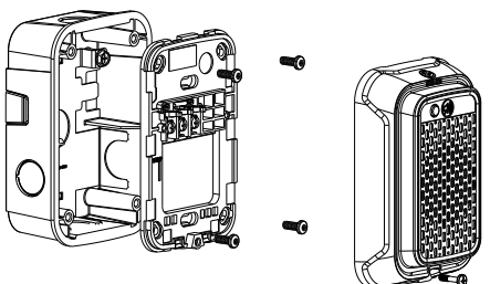
FIGURE 10. COMPACT WALL MOUNT LOW-FREQUENCY SOUNDER WITH LED ALARM INDICATOR AND SILENCE SWITCH, IN SURFACE-MOUNT BACK BOX
