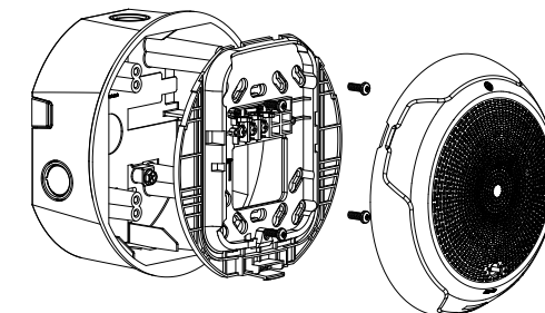
FIGURE 6. CEILING MOUNT LOW-FREQUENCY SOUNDER WITH SURFACE-MOUNT BACK BOX (SOUNDER STROBE SHOWN)
