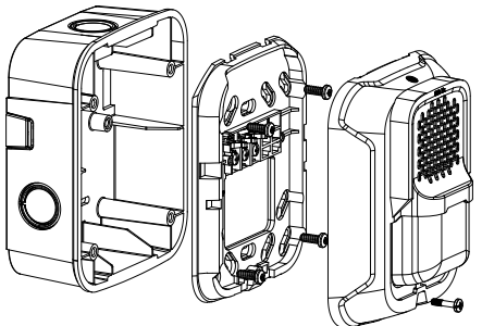
FIGURE 9. COMPACT WALL MOUNT LOW-FREQUENCY SOUNDER SOUNDER WITH LED ALARM INDICATOR AND SILENCE SWITCH, IN JUNCTION BOX
