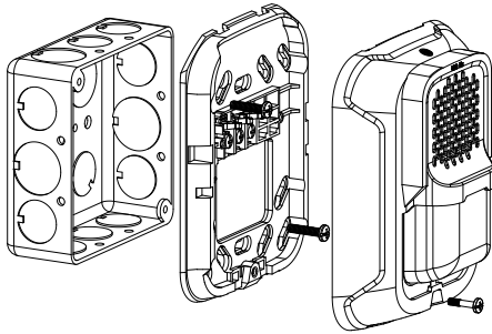
FIGURE 8. WALL MOUNT LOW-FREQUENCY SOUNDER STROBE WITH SURFACE-MOUNT BACK BOX
